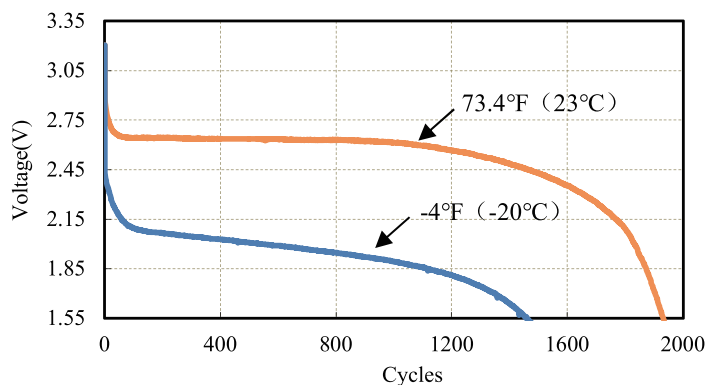
900mA (3s on/27s off) at 73.4°F & -4°F (23°C & -20°C)
