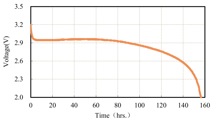
10mA continuous discharge to 2.0V at 73.4°F (23°C)
