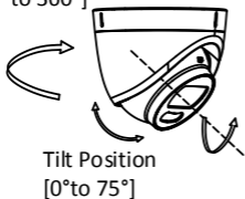
Figure 2-4 3-axis Adjustment
