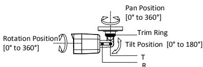
Figure 2-2 3-Axis Adjustment
