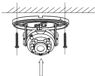
Figure 2-15 Attach the Mounting Base to the Ceiling
