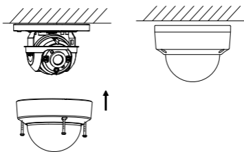
Figure 2-11 Bubble Reinstallation
