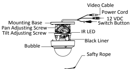
Figure 1-3 Overview of Type III Camera
