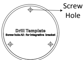
Figure 2-4 Drill Template
