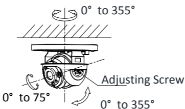
Figure 2-10 Type I Camera 2-Axis Adjustment
