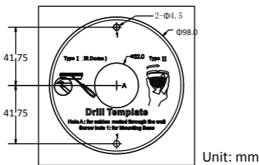
Figure 2-14 Drill Template
