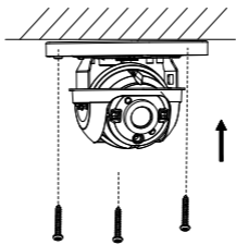
Figure 2-9 Fix the Mounting Base
