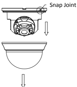
Figure 2-13 Remove the Bubble
