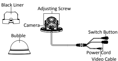
Figure 1-4 Overview of Type III Camera
