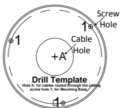
Figure 2-7 Drill Template
