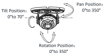
Figure 2-16 3-axis Adjustment
