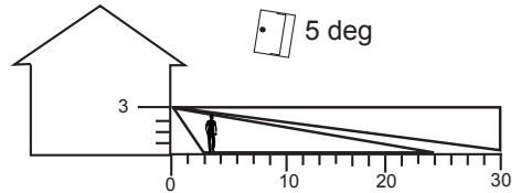
Figure 2: Sensor 3m high, 5 degree tilt, 30m range
