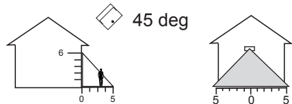
Figure 5: Sensor 6m high, 45 degree tilt, 5m range
