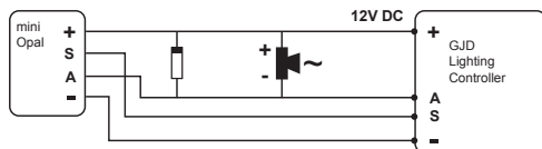
Figure 9: Piezo buzzer wiring diagram
