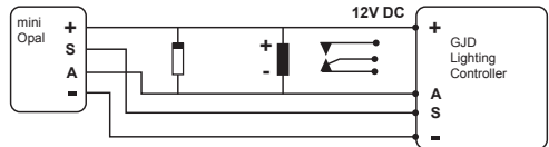
Figure 8: External relay wiring diagram
