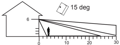
Figure 3: Sensor 6m high, 15 degree tilt, 30m range
