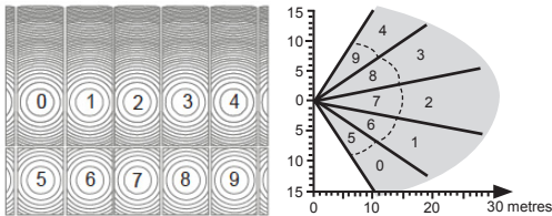
Figure 4: Sensor 1.5m high, -5 degree tilt, 30m range
