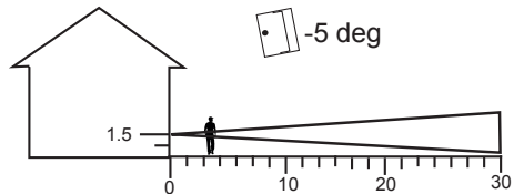
Figure 4: Sensor 1.5m high, -5 degree tilt, 30m range
