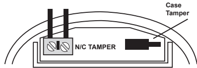
Figure 7: mini Opal tamper board
