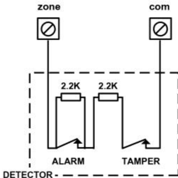
DOUBLE EOL RESISTOR ZONE CONFIGURATION
