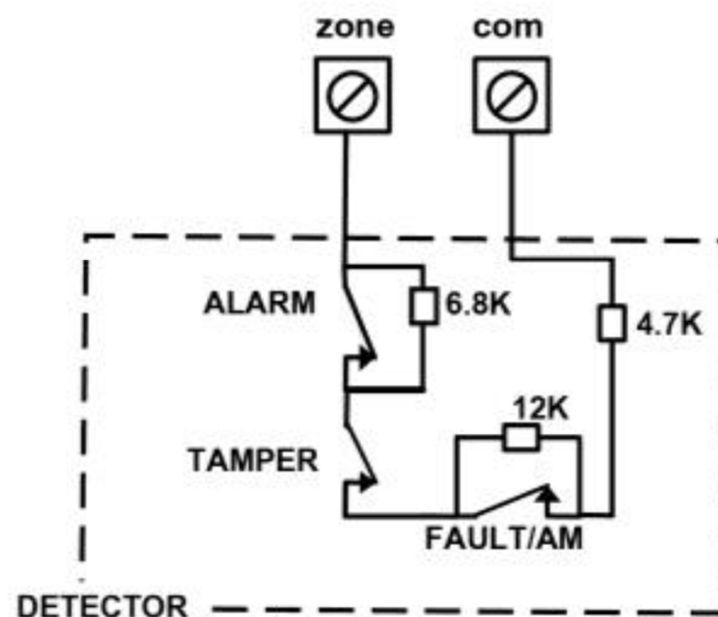
TRIPLE EOL RESISTOR ZONE CONFIGURATION
